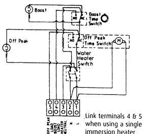
Internal circuit diagram of E7 QUARTZ.
